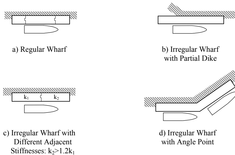
Figure 4-13: Horizontal Marginal Wharf Configurations
