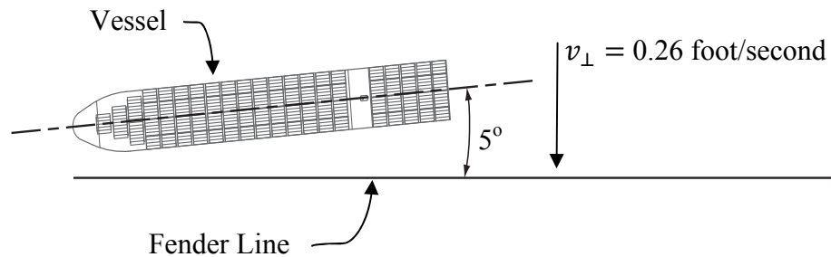
Figure 3-3: Vessel Berthing
